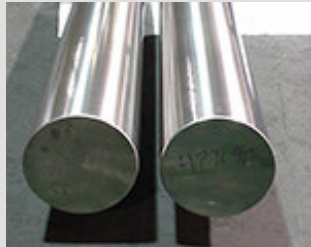
Grinding, Polishing, & Straightening of Stainless Steel Boat Propeller Shafts for the Marine Industry
